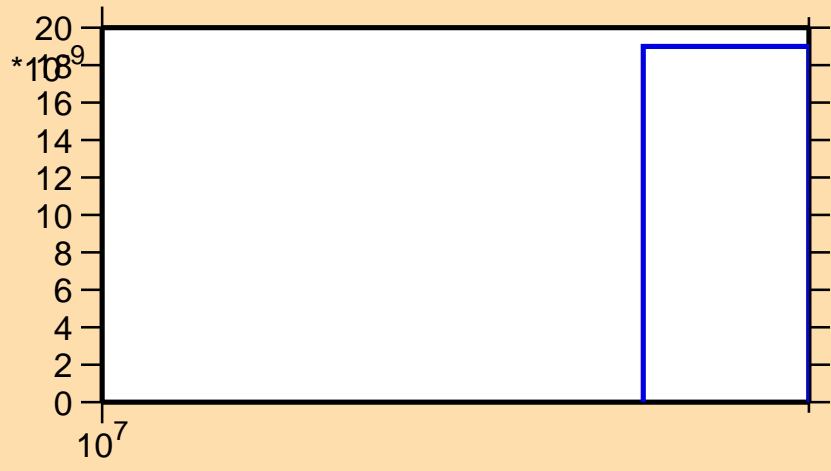
\sigma vs. E for ^{67}\text{Cu}(n,2np)
