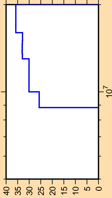
\Delta\sigma/\sigma vs. E for ^{67}\text{Cu}(n,\gamma)
