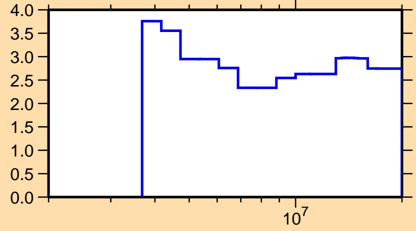
\Delta\sigma/\sigma vs. E for ^{67}\text{Cu}(n,n\text{onel.})
