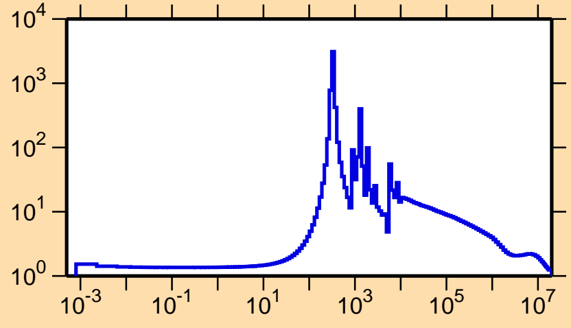
\sigma vs. E for ^{67}\text{Cu}(n,\text{el.})
