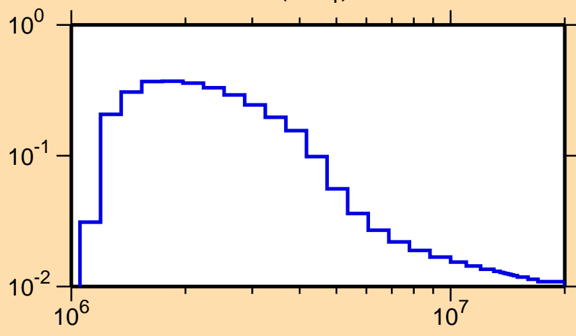
\sigma vs. E for ^{67}\text{Cu}(n,n_1)
