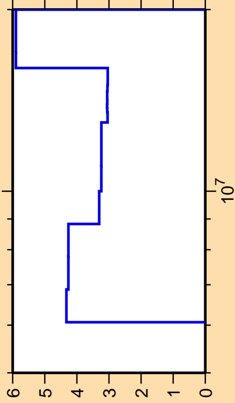
\Delta\sigma/\sigma vs. E for ^{68}\text{Cu}(n,2n)
