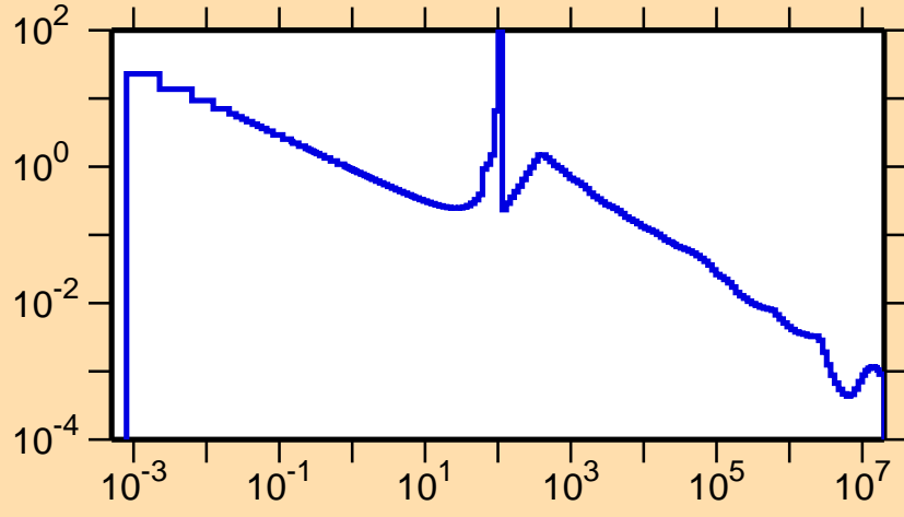
\sigma vs. E for ^{68}\text{Cu}(n,\gamma)
