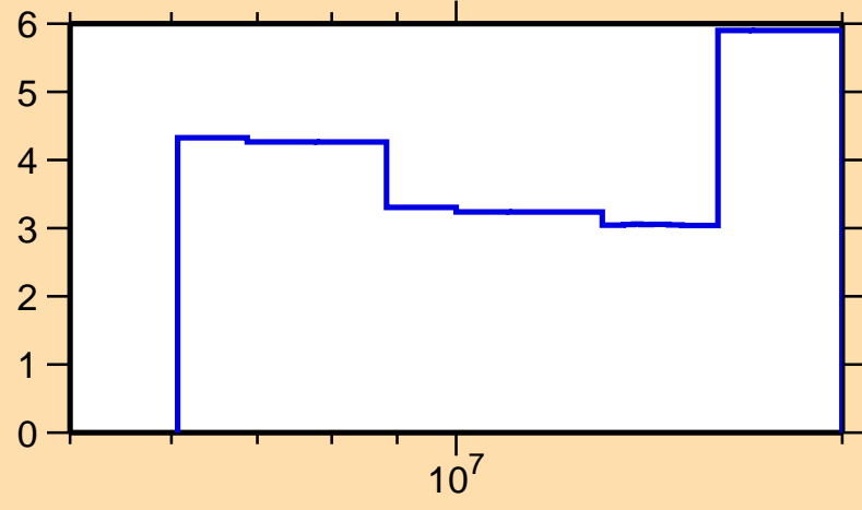
\Delta\sigma/\sigma vs. E for ^{68}\text{Cu}(n,2n)
