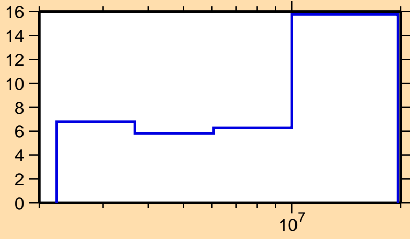
\Delta\sigma/\sigma vs. E for ^{68}\text{Cu}(n,ncont.)
