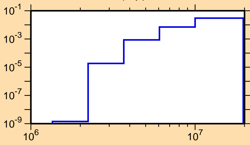
\sigma vs. E for ^{68}\text{Cu}(n,p)
