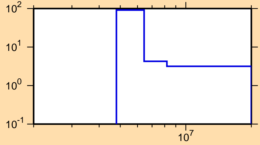
\Delta\sigma/\sigma vs. E for ^{68}\text{Cu}(n,2n)
