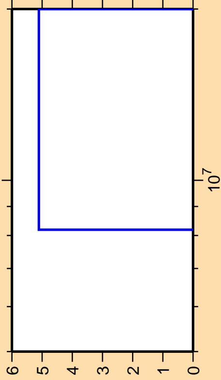
\Delta\sigma/\sigma vs. E for ^{68}\text{Cu}(n,2n\alpha)
