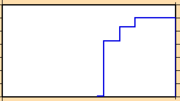
\sigma vs. E for ^{68}\text{Cu}(n,3n)
