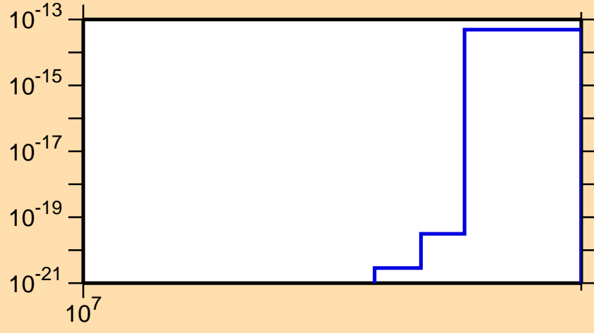
\sigma vs. E for ^{68}\text{Cu}(n,\text{He}3)
