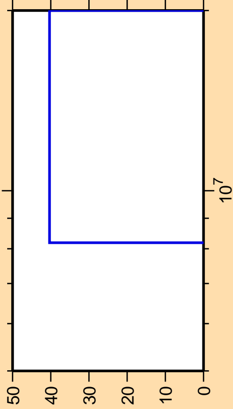
\Delta\sigma/\sigma vs. E for ^{68}\text{Cu}(n,nd)
