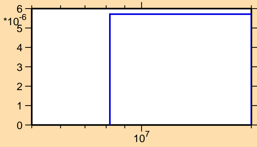
\sigma vs. E for ^{68}\text{Cu}(n,nd)
