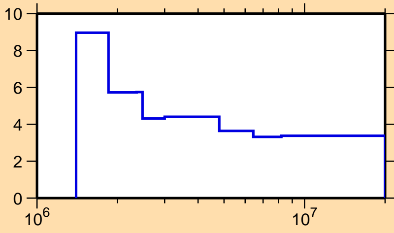
\Delta\sigma/\sigma vs. E for ^{68}\text{Cu}(n,n\text{onel.})
