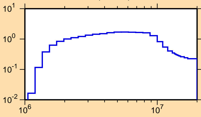
\sigma vs. E for ^{69}\text{Cu}(n,\text{inel.})
