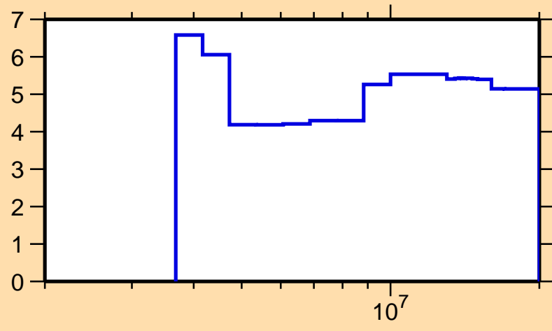
\Delta\sigma/\sigma vs. E for ^{69}\text{Cu}(n,n\text{nonel.})
