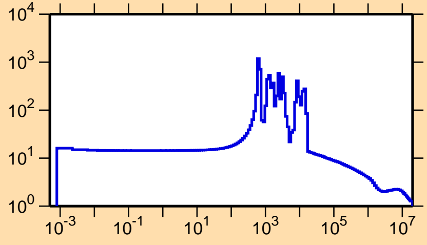
\sigma vs. E for ^{69}\text{Cu}(n,\text{el.})
