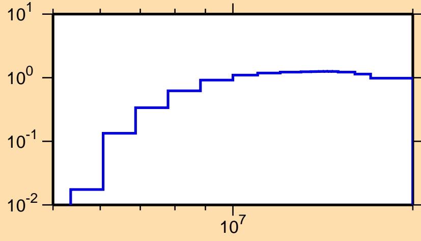
\sigma vs. E for ^{70}\text{Cu}(n,2n)
