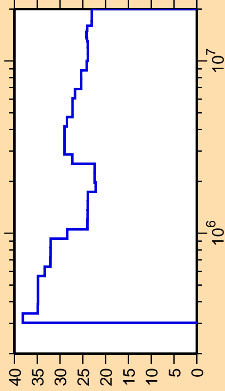
\Delta\sigma/\sigma vs. E for ^{70}\text{Cu}(n,n_4)
