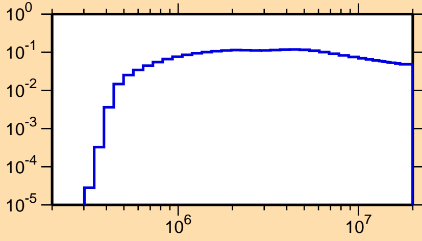
\sigma vs. E for ^{70}\text{Cu}(n,n_4)
