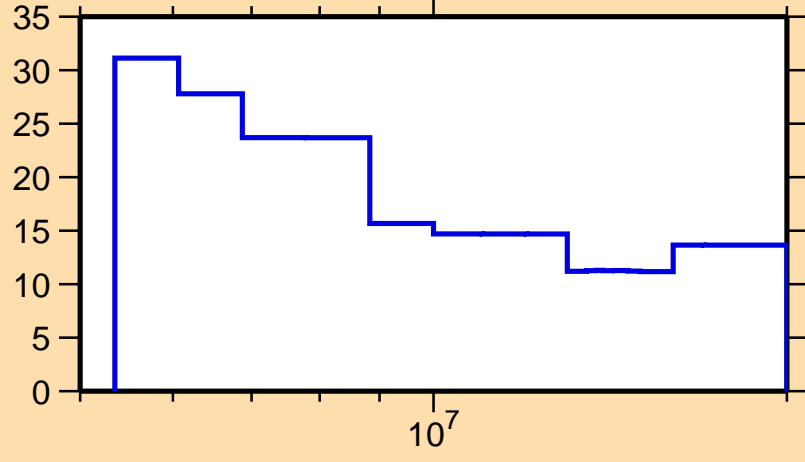
\Delta\sigma/\sigma vs. E for ^{70}\text{Cu}(n,2n)
