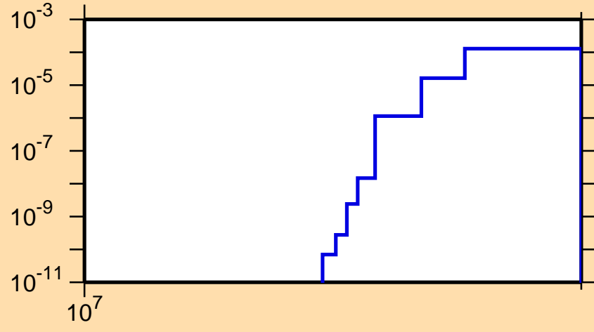
\sigma vs. E for ^{70}\text{Cu}(n,\text{nd})
