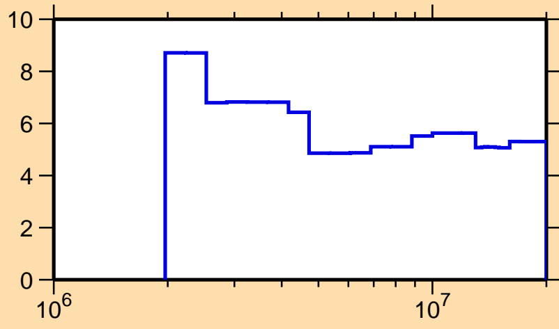
\Delta\sigma/\sigma vs. E for ^{70}\text{Cu}(n,n\text{onel.})
