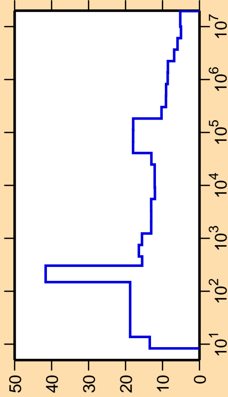
\Delta\sigma/\sigma vs. E for ^{70}\text{Cu}(n,\text{nonel.})
