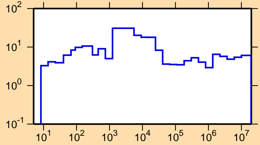
\Delta\sigma/\sigma vs. E for ^{70}\text{Cu}(n,\text{el.})
