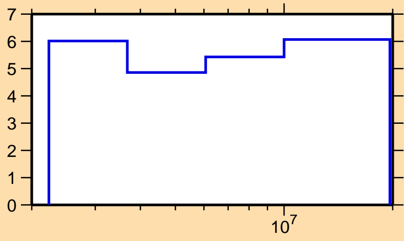
\Delta\sigma/\sigma vs. E for ^{70}\text{Cu}(n,el.)
