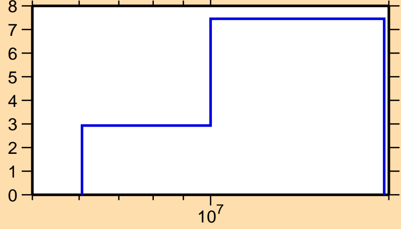
\Delta\sigma/\sigma vs. E for ^{71}\text{Cu}(n,\text{tot.})
