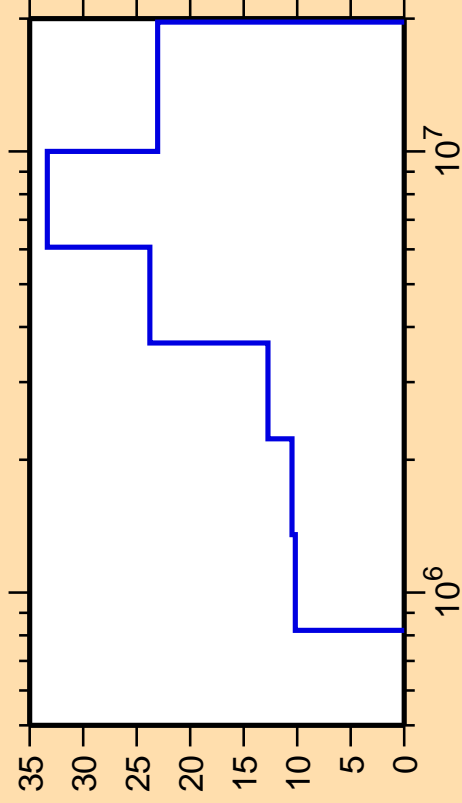
\Delta\sigma/\sigma vs. E for ^{71}\text{Cu}(n,n_3)
