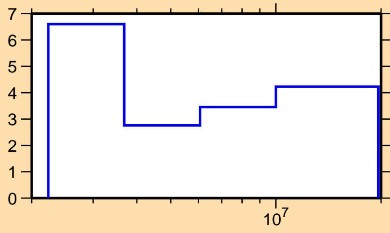
\Delta\sigma/\sigma vs. E for ^{72}\text{Cu}(n,n\text{onel.})
