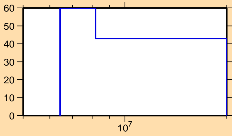
\Delta\sigma/\sigma vs. E for ^{72}\text{Cu}(n,p)
