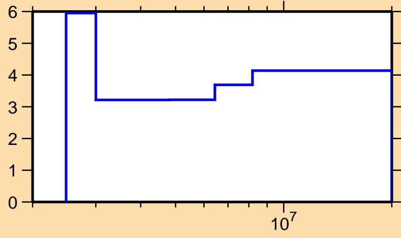
\Delta\sigma/\sigma vs. E for ^{72}\text{Cu}(n,\text{nonel.})
