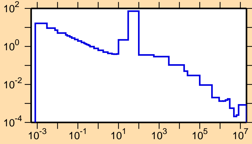
\sigma vs. E for ^{72}\text{Cu}(n,\gamma)
