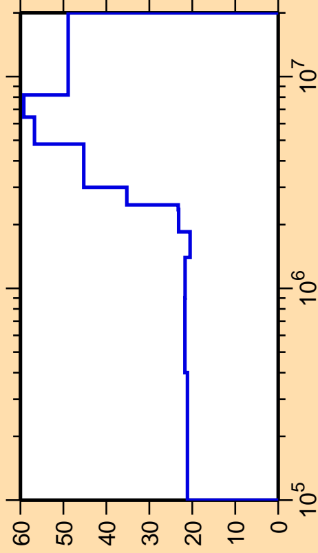
\Delta\sigma/\sigma vs. E for ^{72}\text{Cu}(n,n_1)
