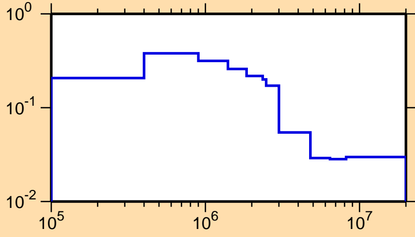
\sigma vs. E for ^{72}\text{Cu}(n,n_1)
