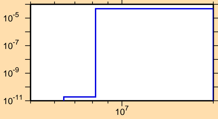
\sigma vs. E for ^{72}\text{Cu}(n,\alpha)
