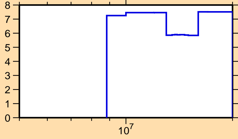
\Delta\sigma/\sigma vs. E for ^{73}\text{Cu}(n,\text{nonel.})
