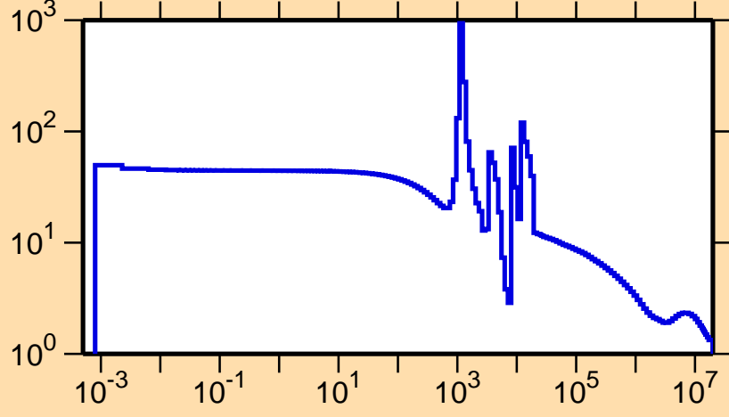
\sigma vs. E for ^{73}\text{Cu}(n,\text{el.})
