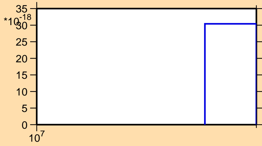
\sigma vs. E for ^{73}\text{Cu}(n,2n\alpha)
