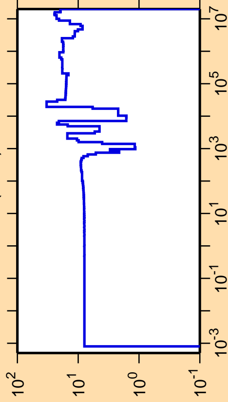
\Delta\sigma/\sigma vs. E for ^{73}\text{Cu}(n,\text{el.})
