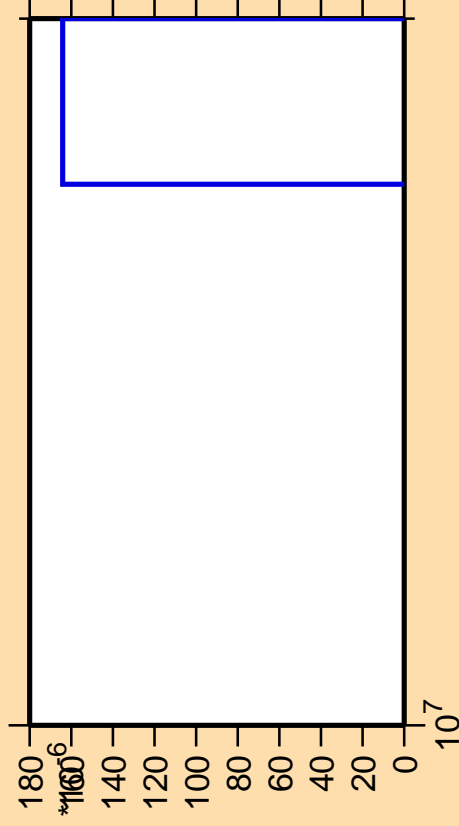
\Delta\sigma/\sigma vs. E for ^{73}\text{Cu}(n,2n\alpha)
