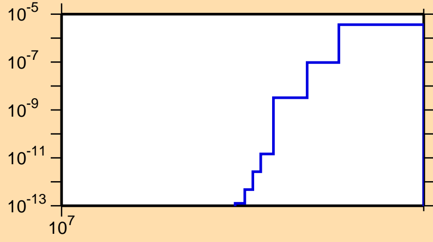
\sigma vs. E for ^{73}\text{Cu}(n,n\alpha)
