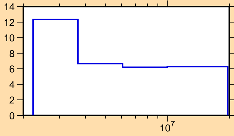
\Delta\sigma/\sigma vs. E for ^{73}\text{Cu}(n,n\text{nonel.})
