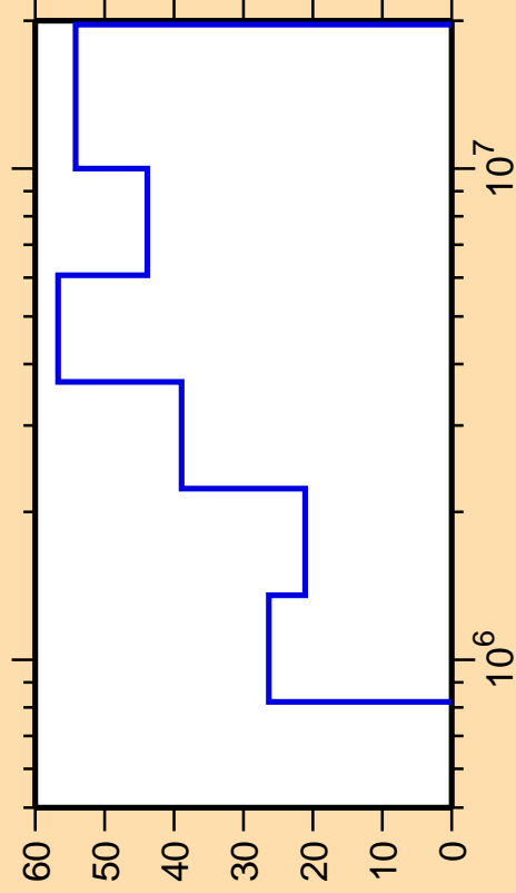
\Delta\sigma/\sigma vs. E for ^{73}\text{Cu}(n,n_2)
