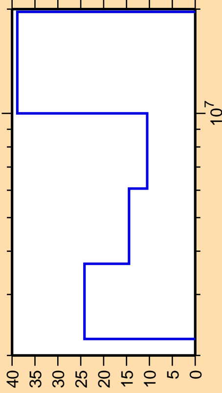
\Delta\sigma/\sigma vs. E for ^{73}\text{Cu}(n,n\text{cont.})
