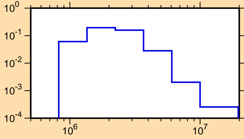
\sigma vs. E for ^{73}\text{Cu}(n,n_2)
