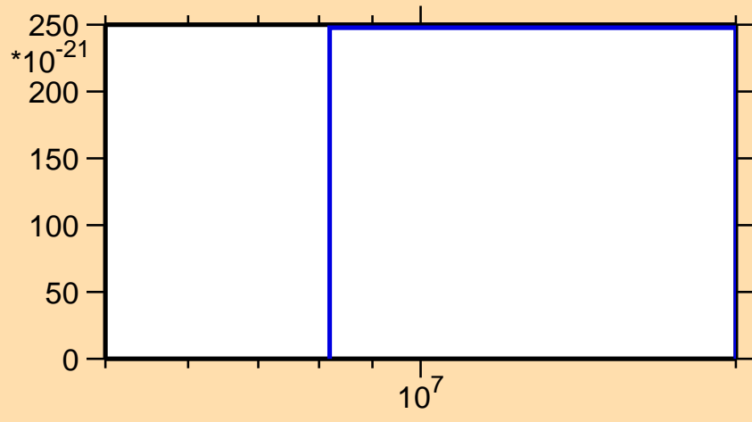
\sigma vs. E for ^{73}\text{Cu}(n,2n\alpha)
