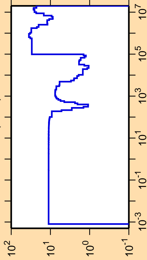
\Delta\sigma/\sigma vs. E for ^{75}\text{Cu}(n,\text{el.})
