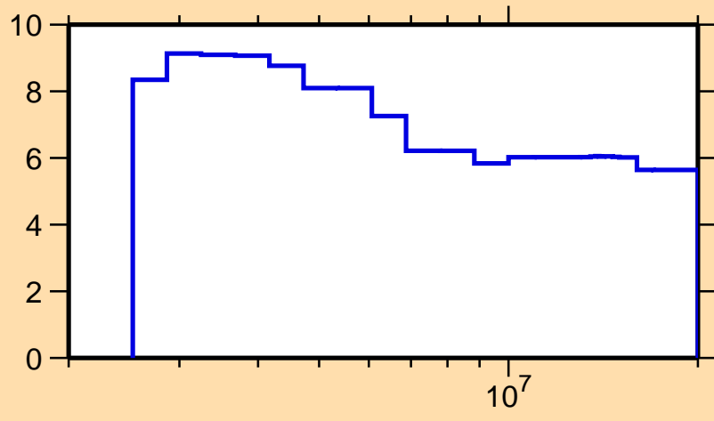
\Delta\sigma/\sigma vs. E for ^{75}\text{Cu}(n,n\text{onel.})
