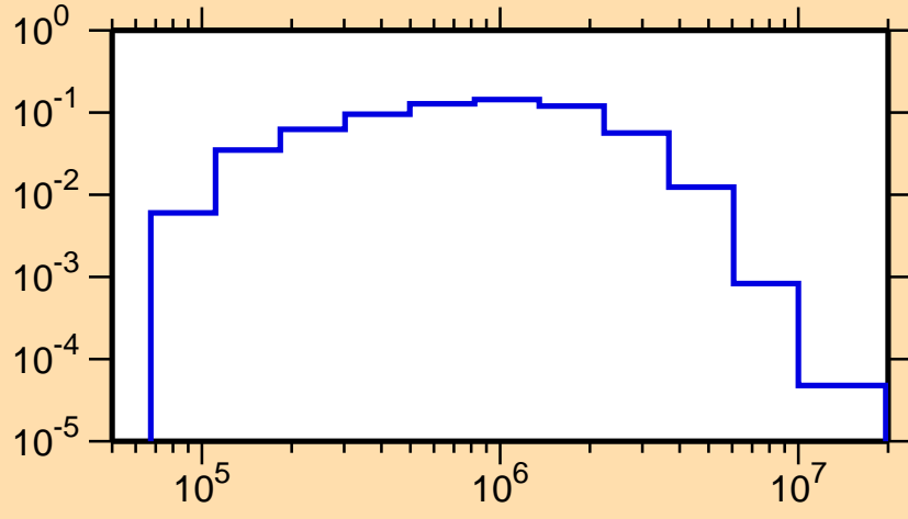
\sigma vs. E for ^{75}\text{Cu}(n,n_1)
