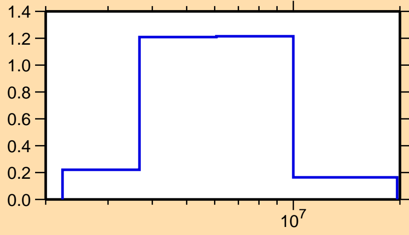
\sigma vs. E for ^{75}\text{Cu}(n,n\text{cont.})
