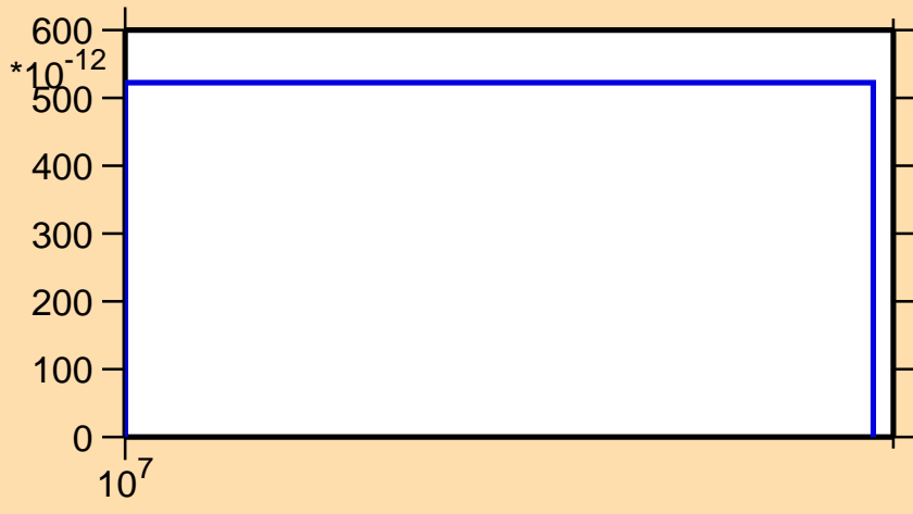
\sigma vs. E for ^{75}\text{Cu}(n,n\alpha)
