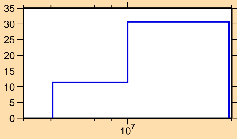
\Delta\sigma/\sigma vs. E for ^{75}\text{Cu}(n,ncont.)
