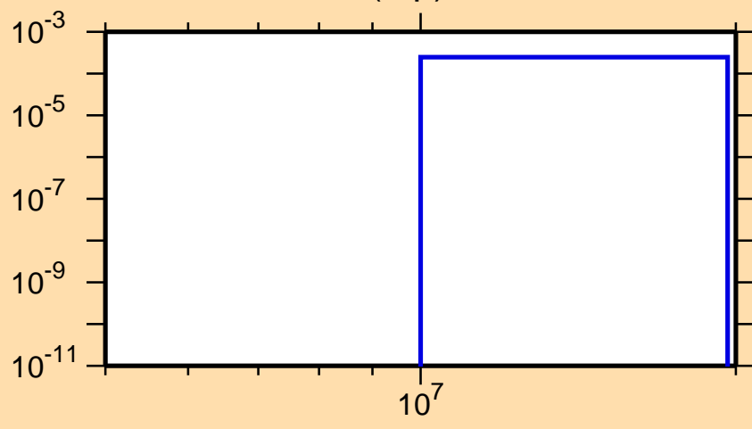
\sigma vs. E for ^{75}\text{Cu}(n,p)
