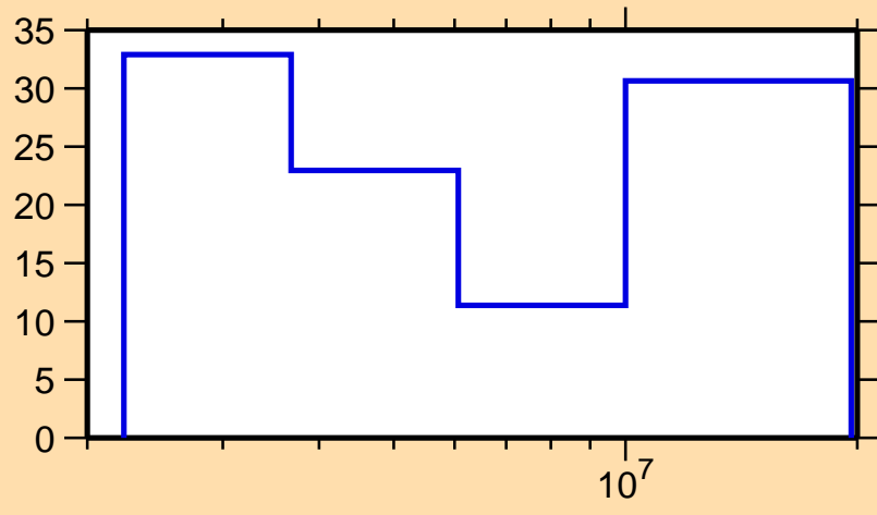
\Delta\sigma/\sigma vs. E for ^{75}\text{Cu}(n,n\text{cont.})
