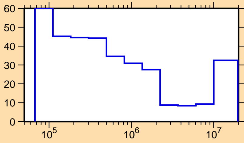
\Delta\sigma/\sigma vs. E for ^{75}\text{Cu}(n,\text{inel.})
