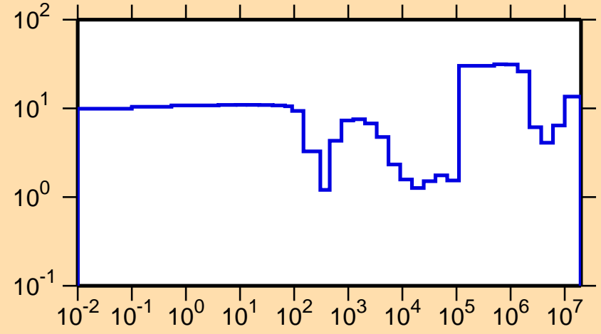
\Delta\sigma/\sigma vs. E for ^{75}\text{Cu}(n,\text{tot.})
