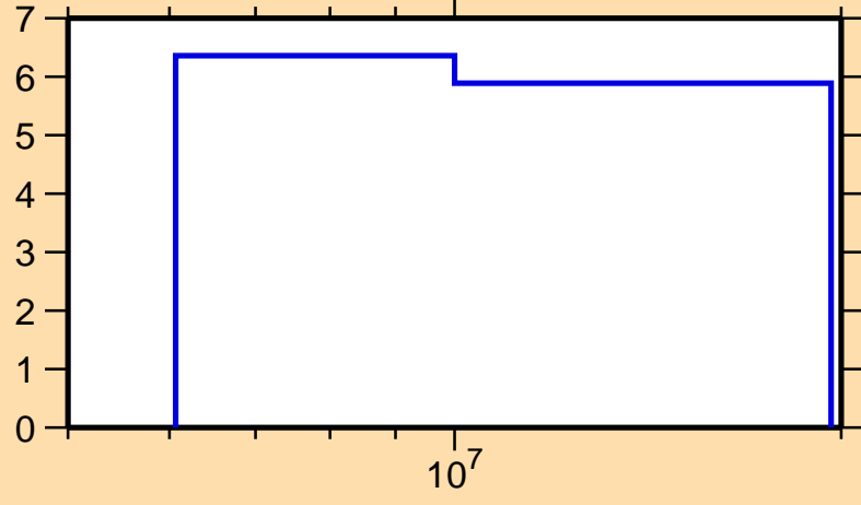
\Delta\sigma/\sigma vs. E for ^{75}\text{Cu}(n,\text{nonel.})
