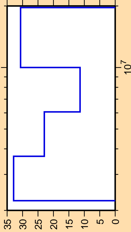
\Delta\sigma/\sigma vs. E for ^{75}\text{Cu}(n,n\text{cont.})
