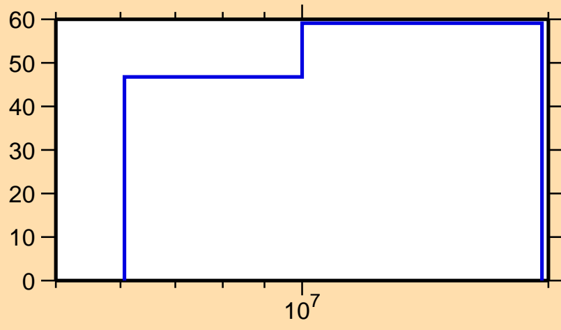
\Delta\sigma/\sigma vs. E for ^{75}\text{Cu}(n,n_1)
