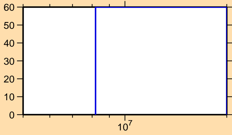
\Delta\sigma/\sigma vs. E for ^{75}\text{Cu}(n,p)
