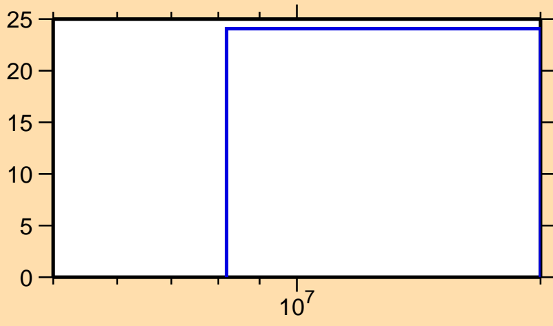
\Delta\sigma/\sigma vs. E for ^{75}\text{Cu}(n,el.)
