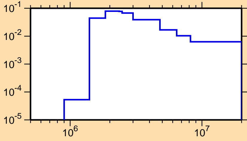
\sigma vs. E for ^{75}\text{Cu}(n,n_4)
