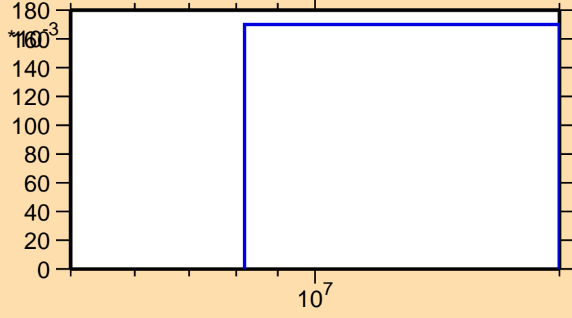
\sigma vs. E for ^{75}\text{Cu}(n,3n)
