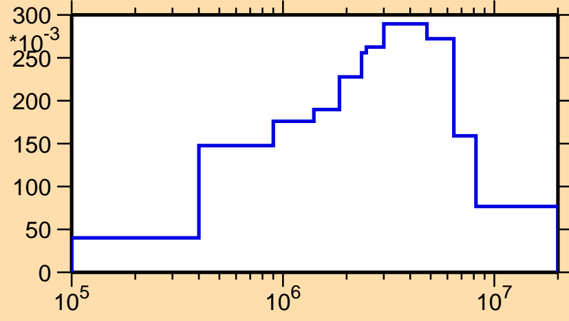
\sigma vs. E for ^{255}\text{Pu}
