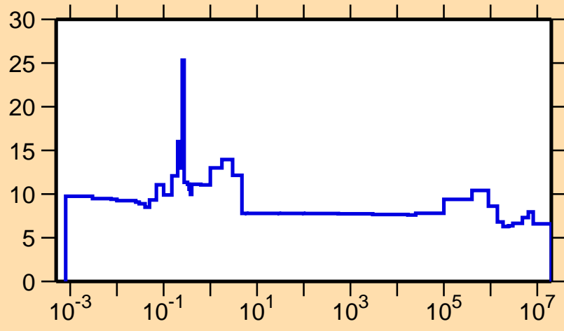
\sigma vs. E for ^{255}
