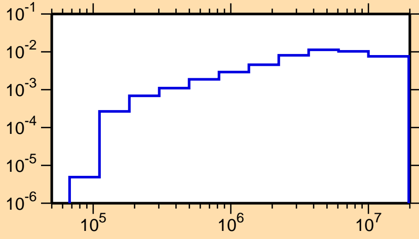
\sigma vs. E for ^{256}_{1}
