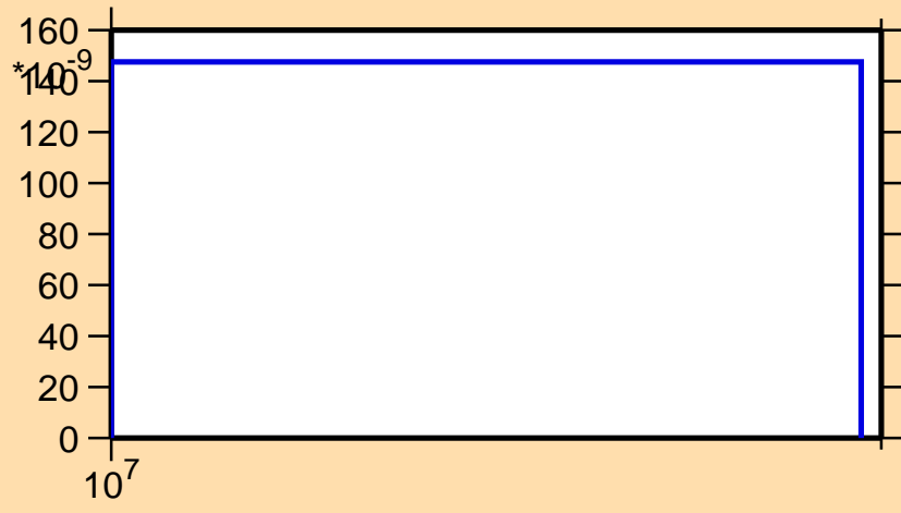
\sigma vs. E for ^{256}\alpha )
