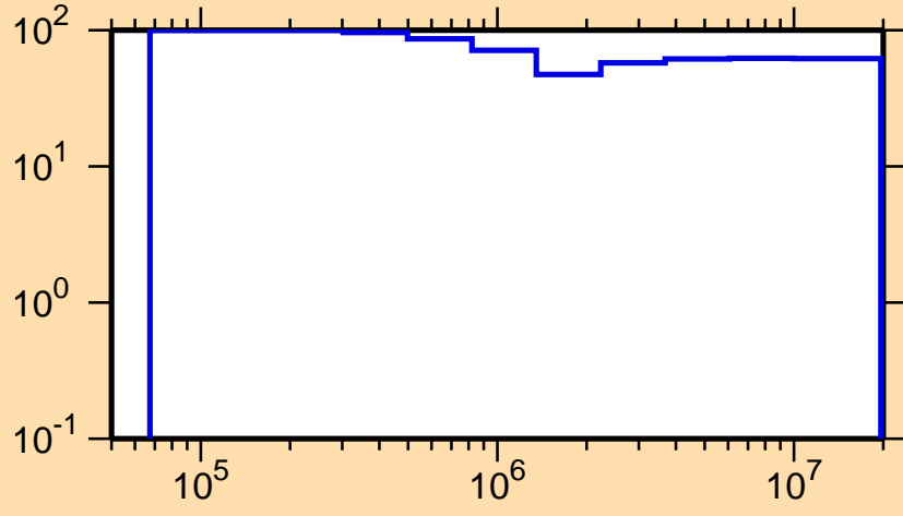
\Delta\sigma/\sigma vs. E for ^{256}_{1}\text{Pa}
