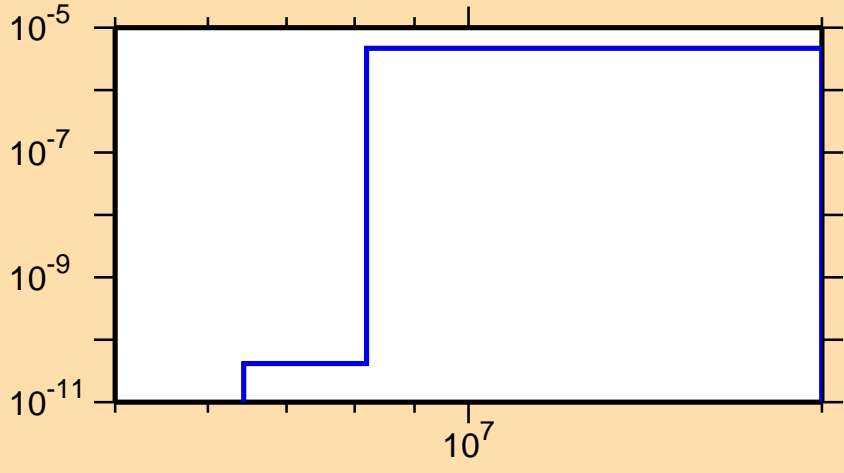
\sigma vs. E for ^{256}\text{He3}
