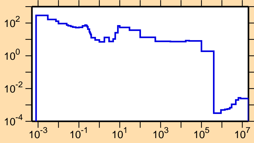
\sigma vs. E for ^{256}\gamma
