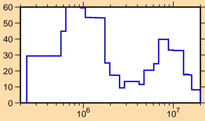
\Delta\sigma/\sigma vs. E for ^{258}\text{Cf}
