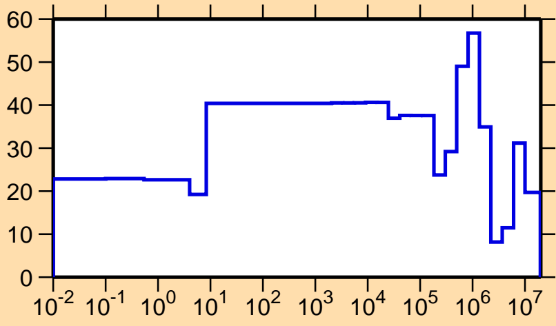
\Delta\sigma/\sigma vs. E for ^{258}\text{Pu}
