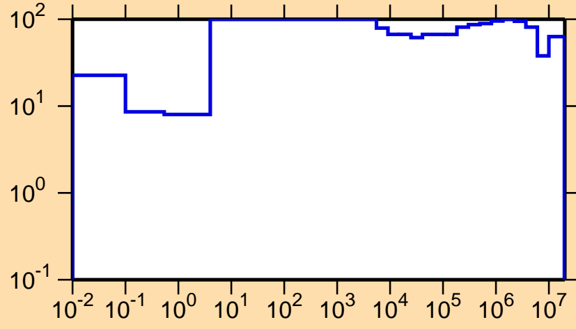
\Delta\sigma/\sigma vs. E for ^{258}\text{Po} ( \gamma )
