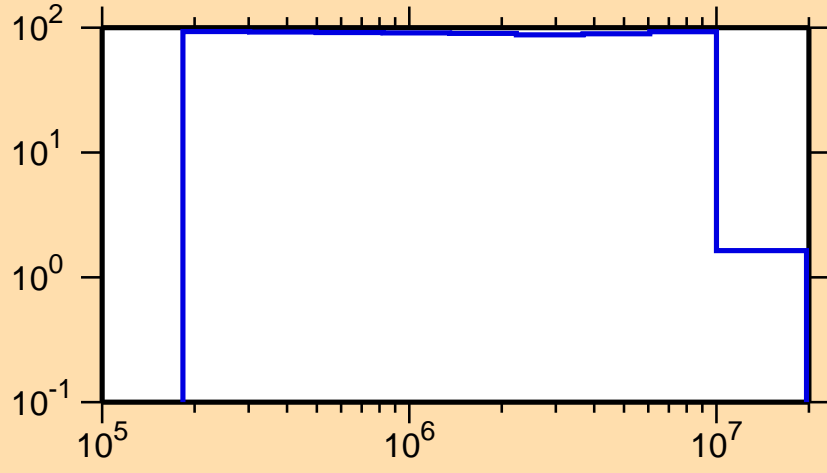
\Delta\sigma/\sigma vs. E for ^{258}_{1}
