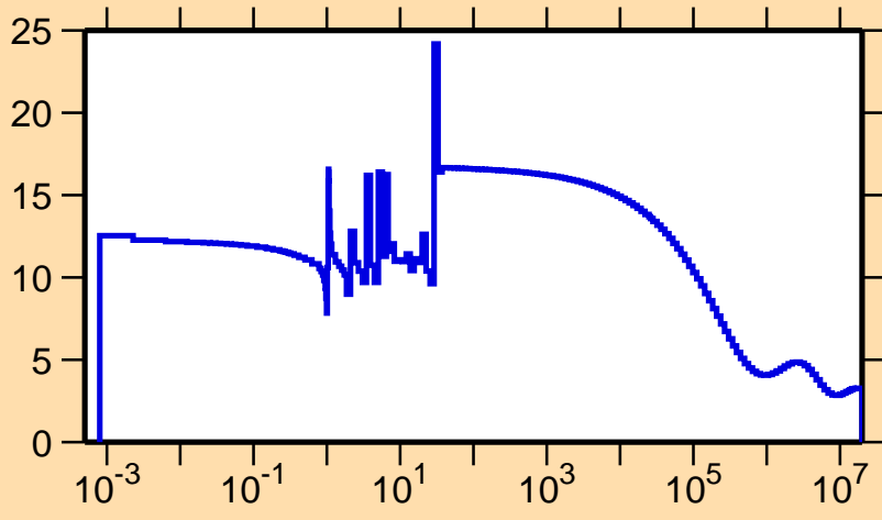
\sigma vs. E for ^{258}
