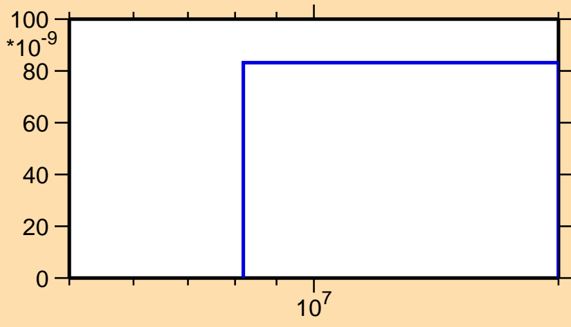
\sigma vs. E for ^{258}\text{He3}
