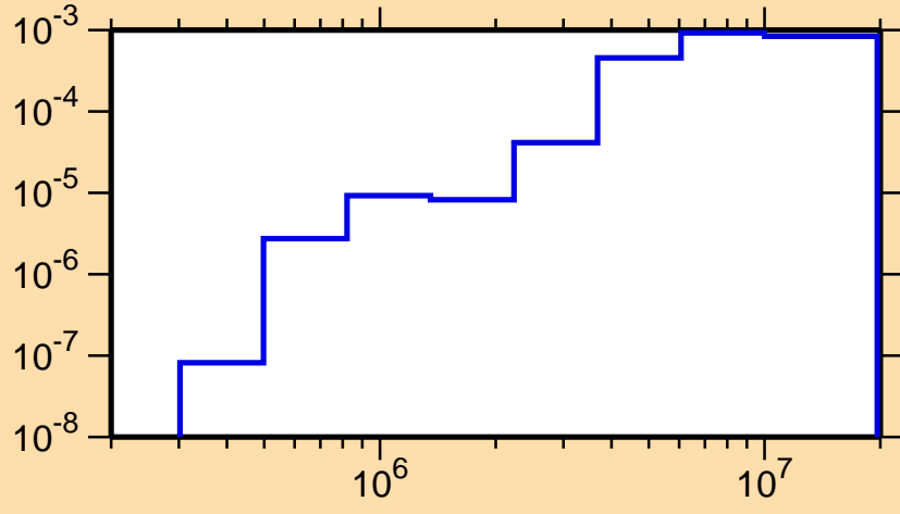
\sigma vs. E for ^{260}_{3}
