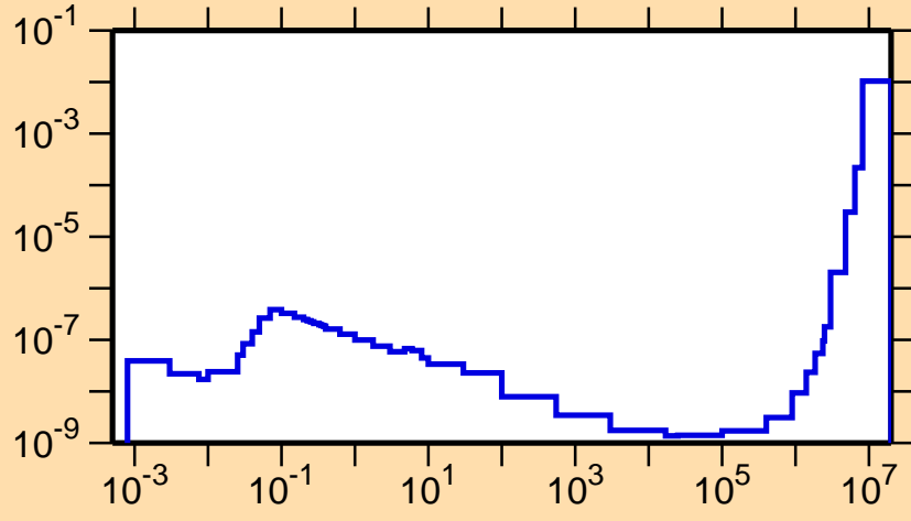
\sigma vs. E for ^{261}\text{Pu}
