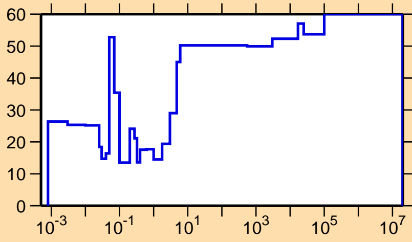
\Delta\sigma/\sigma vs. E for ^{261}\gamma
