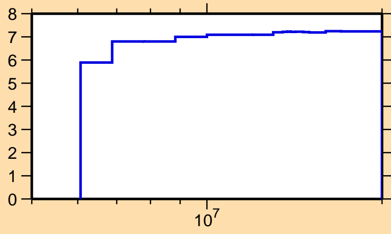
\Delta\sigma/\sigma vs. E for 262
