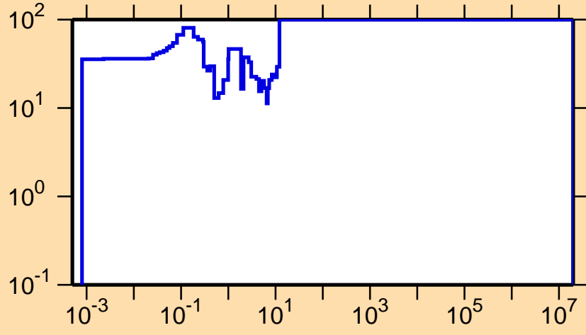
\Delta\sigma/\sigma vs. E for ^{262}\text{Pu}
