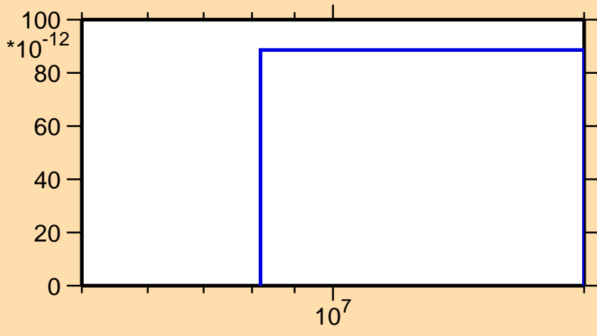
\sigma vs. E for ^{262}\text{He3}
