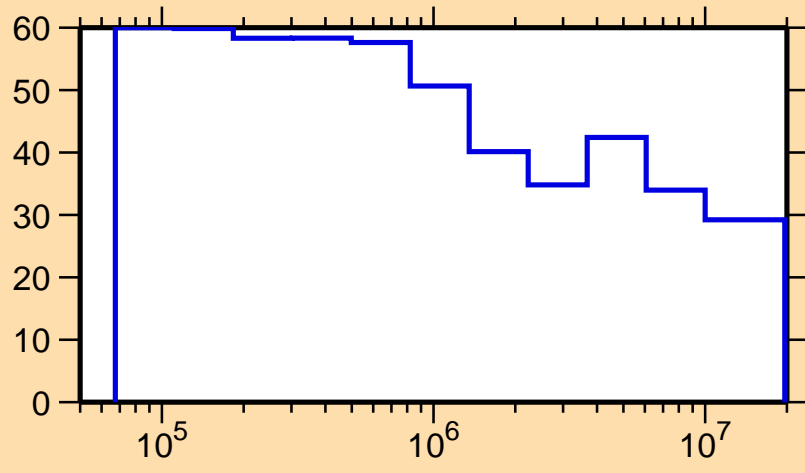
\Delta\sigma/\sigma vs. E for ^{263}_{1}
