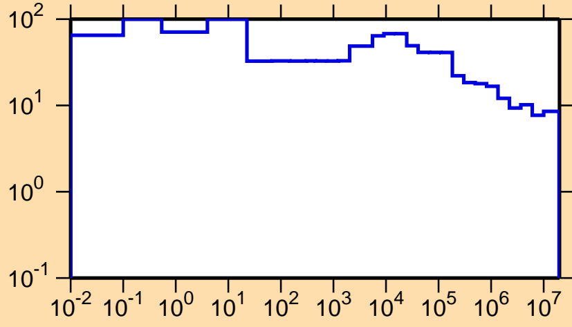
\Delta\sigma/\sigma vs. E for ^{263}\text{Po}
