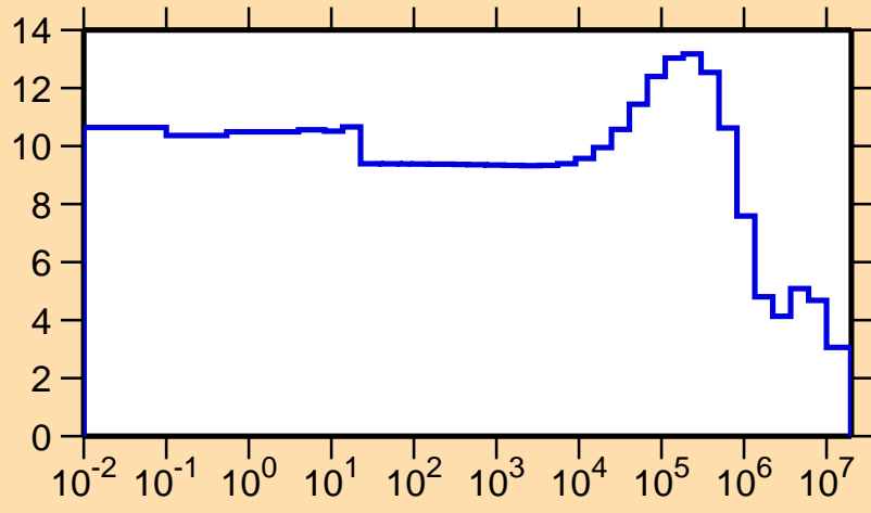
\sigma vs. E for ^{263}
