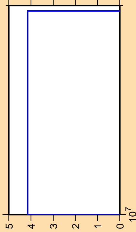
\Delta\sigma/\sigma vs. E for ^{267}\text{He3}
