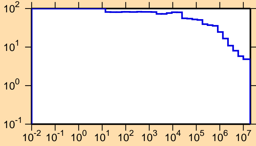
\Delta\sigma/\sigma vs. E for ^{269}\text{Tc}
