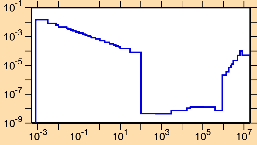
\sigma vs. E for ^{280}\gamma
