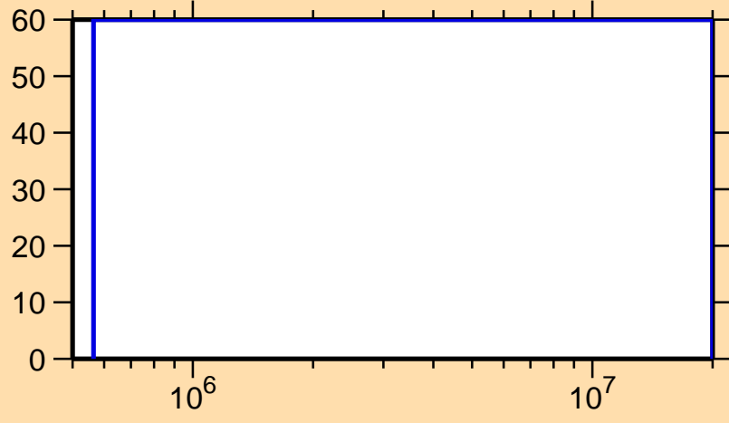
\Delta\sigma/\sigma vs. E for ^{281}_{1}\text{Pm}
