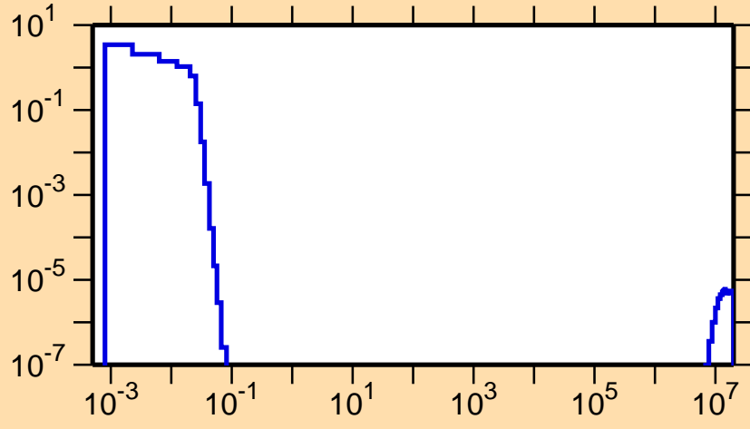
\sigma vs. E for ^{281}\alpha
