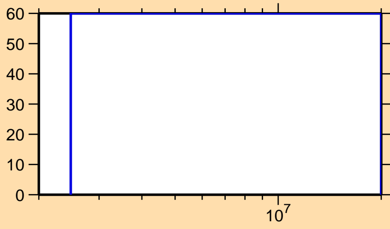
\Delta\sigma/\sigma vs. E for ^{281}_1
