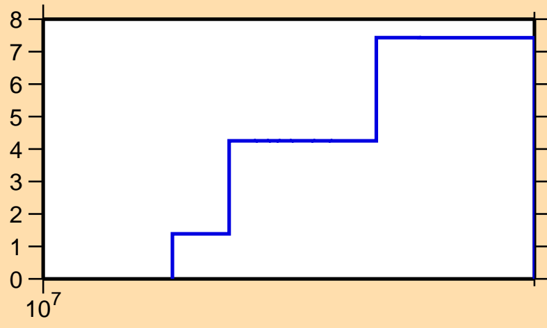
\Delta\sigma/\sigma vs. E for ^{142}\text{Dy}(n,\text{tot.})
