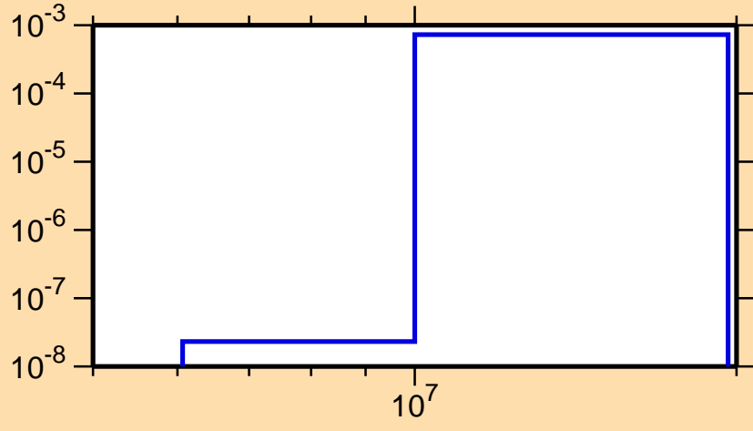
\sigma vs. E for ^{142}\text{Dy}(n,\text{pd})
