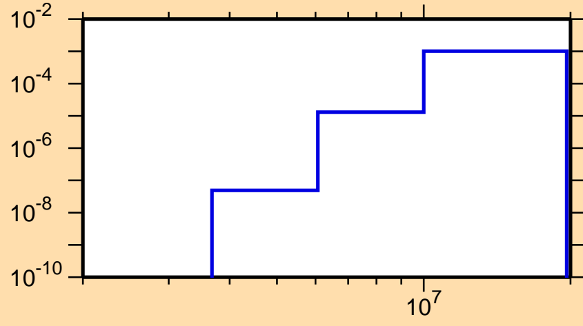
\sigma vs. E for ^{142}\text{Dy}(n,n\alpha)
