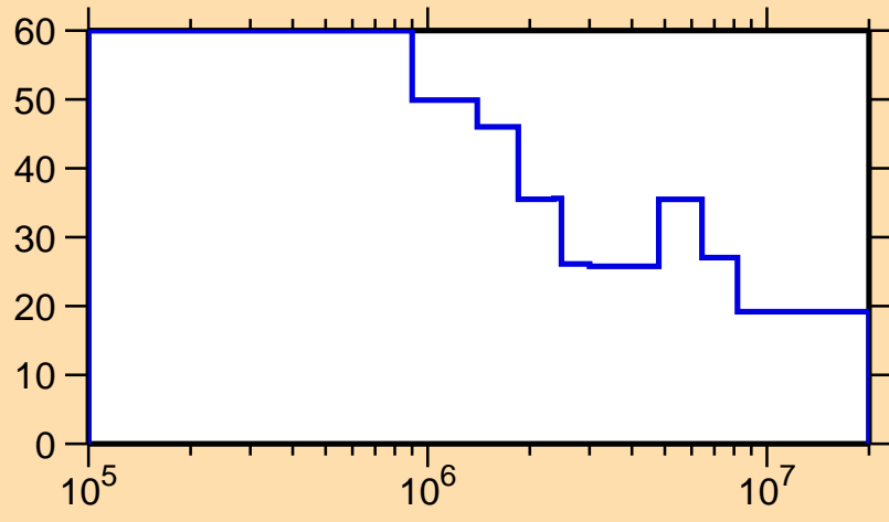
\Delta\sigma/\sigma vs. E for ^{142}\text{Dy}(n,n_1)
