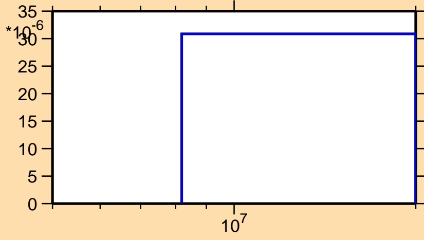
\sigma vs. E for ^{142}\text{Dy}(n,t)
