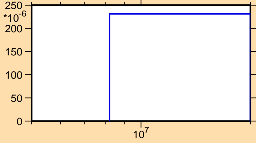
\sigma vs. E for ^{142}\text{Dy}(n,2n)
