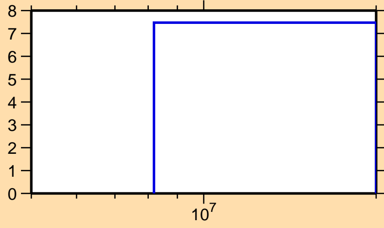
\Delta\sigma/\sigma vs. E for ^{142}\text{Dy}(n,\text{nonel.})
