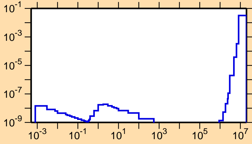
\sigma vs. E for ^{142}\text{Dy}(n,p\alpha)
