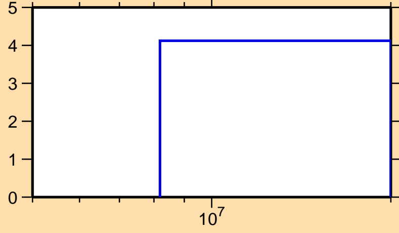
\Delta\sigma/\sigma vs. E for ^{142}\text{Dy}(n,\text{el.})
