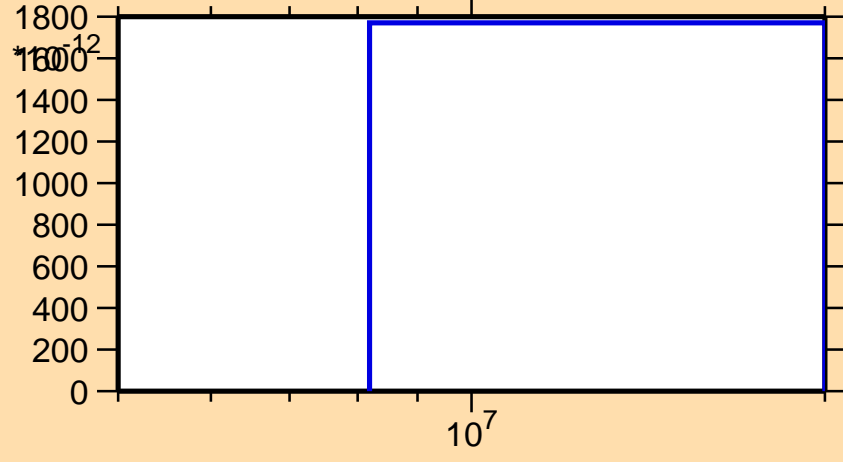
\sigma vs. E for ^{142}\text{Dy}(\text{mt117})
