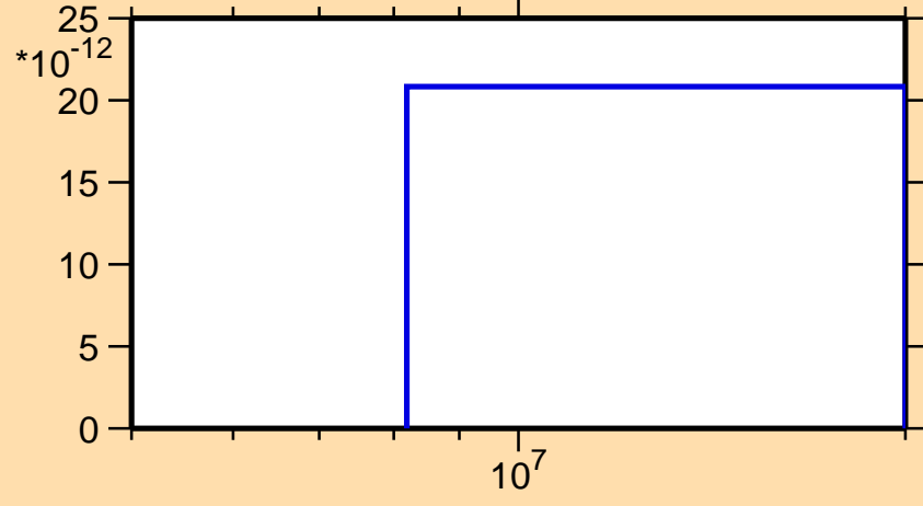
\sigma vs. E for ^{142}\text{Dy}(n,nd)
