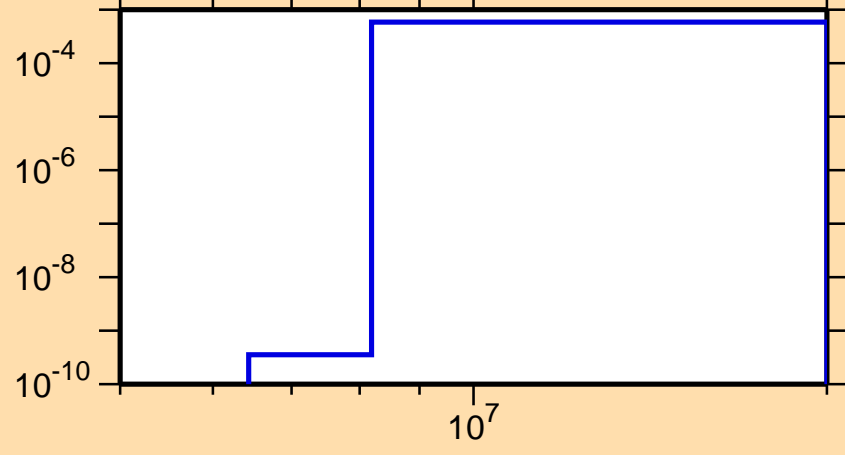
\sigma vs. E for ^{142}\text{Dy}(n,\text{pd})
