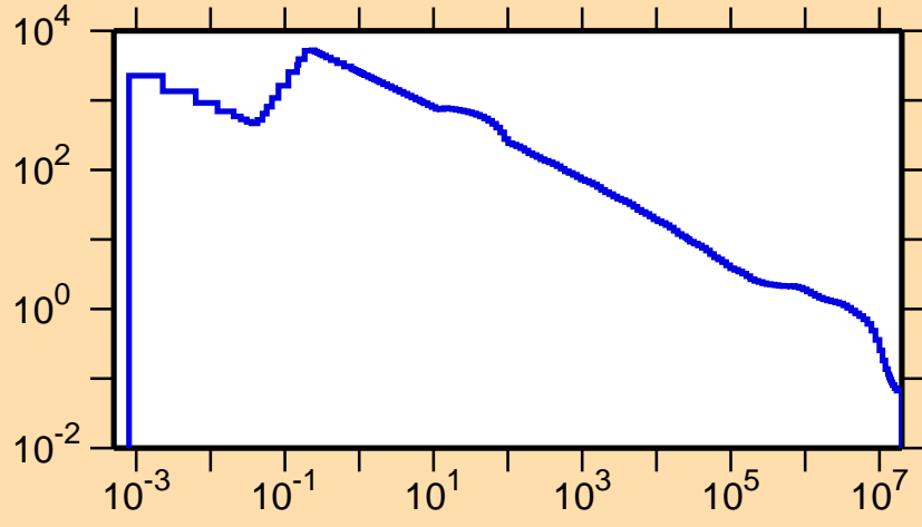
\sigma vs. E for ^{143}\text{Dy}(n,p)
