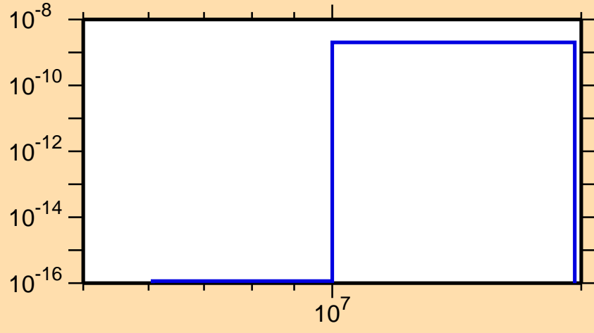
\sigma vs. E for ^{143}\text{Dy}(\text{mt117})
