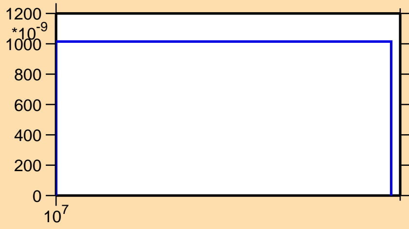
\sigma vs. E for ^{143}\text{Dy}(n,2np)
