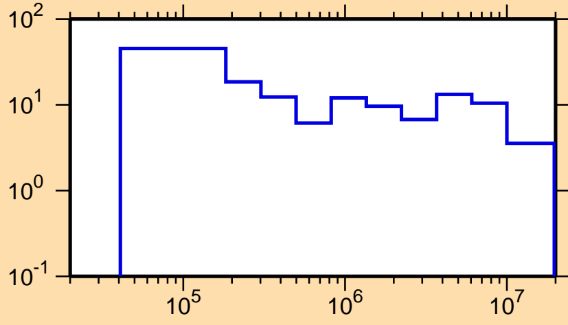
\Delta\sigma/\sigma vs. E for ^{143}\text{Dy}(n,\text{tot.})
