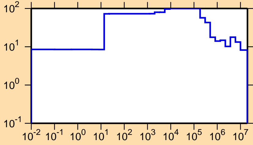
\Delta\sigma/\sigma vs. E for ^{143}\text{Dy}(n,\text{el.})
