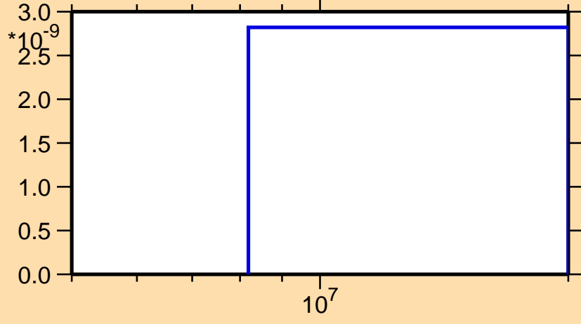
\sigma vs. E for ^{143}\text{Dy}(n,nd)
