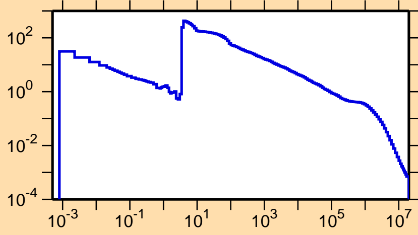
\sigma vs. E for ^{143}\text{Dy}(n,\gamma)
