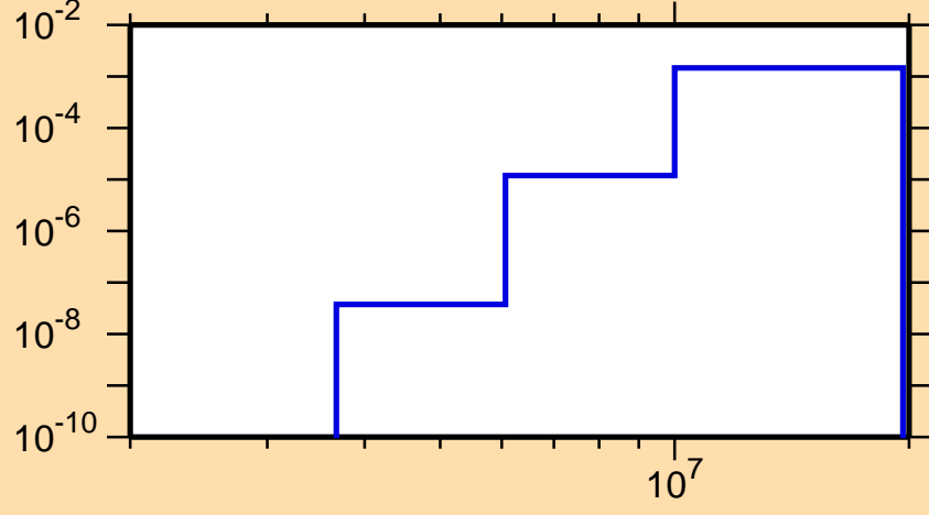
\sigma vs. E for ^{143}\text{Dy}(n,n\alpha)
