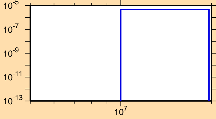
\sigma vs. E for ^{143}\text{Dy}(n,pt)
