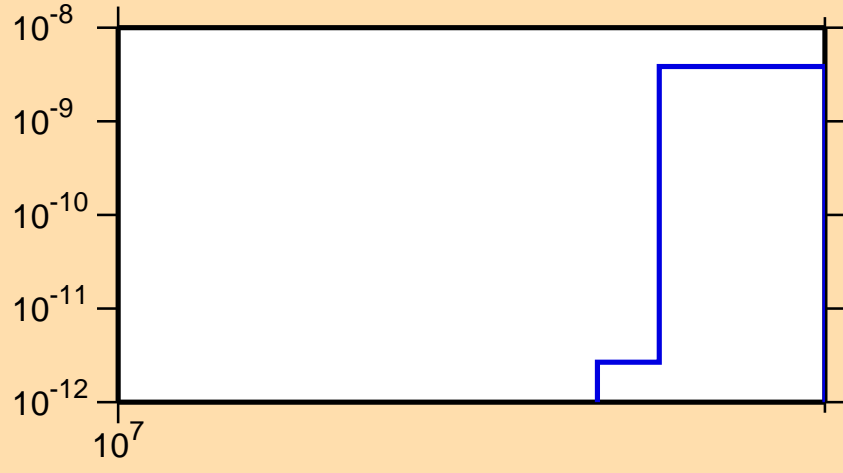
\sigma vs. E for ^{144}\text{Dy}(n,nd)
