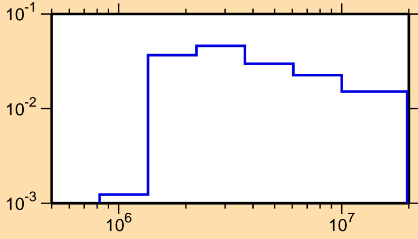
\sigma vs. E for ^{144}\text{Dy}(n,n_2)
