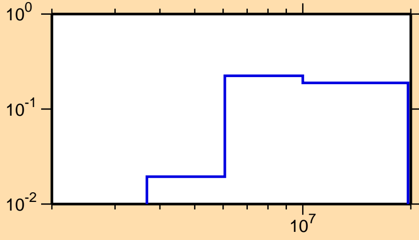
\sigma vs. E for ^{144}\text{Dy}(n,n\text{cont.})
