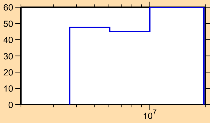
\Delta\sigma/\sigma vs. E for ^{144}\text{Dy}(n,n\text{cont.})
