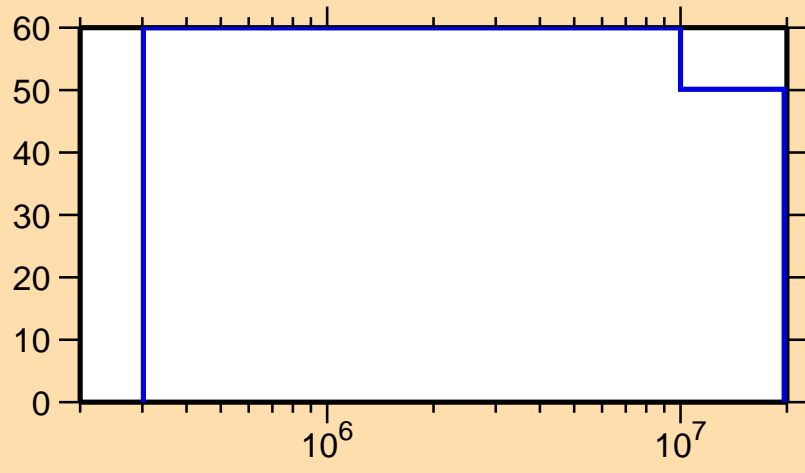
\Delta\sigma/\sigma vs. E for ^{144}\text{Dy}(n,n_1)
