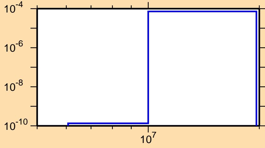
\sigma vs. E for ^{144}\text{Dy}(n,\text{pd})
