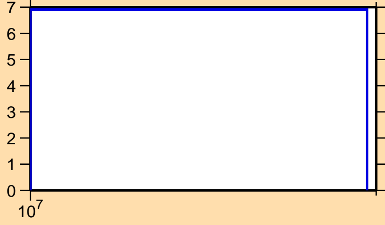
\Delta\sigma/\sigma vs. E for ^{144}\text{Dy}(n,\text{el.})
