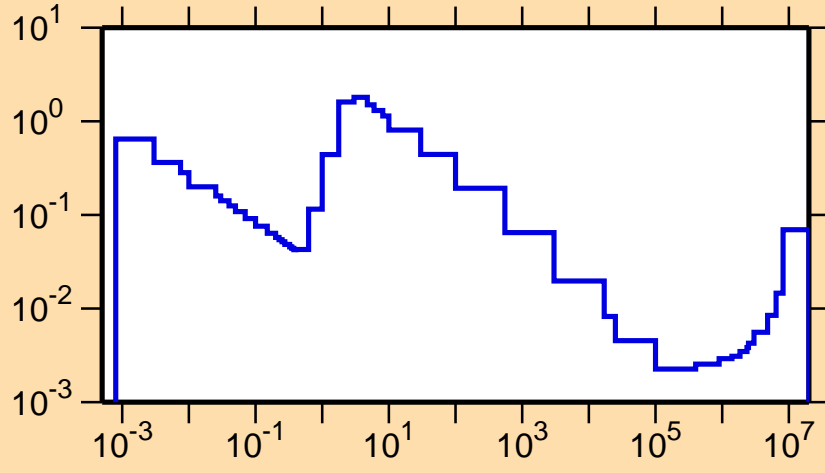
\sigma vs. E for ^{144}\text{Dy}(n,\alpha)
