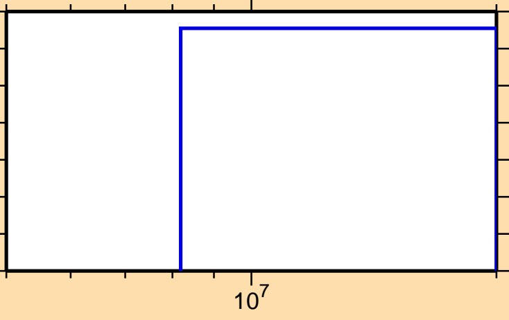
\sigma vs. E for ^{144}\text{Dy} (mt 45)
