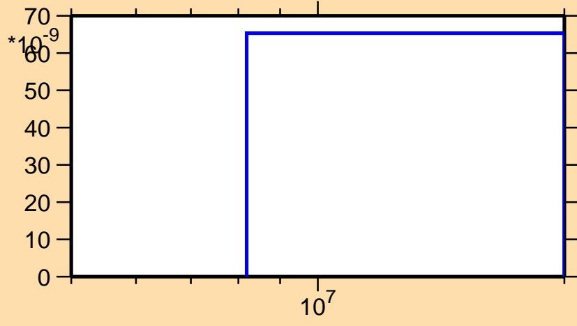
\sigma vs. E for ^{145}\text{Dy} (mt 45)
