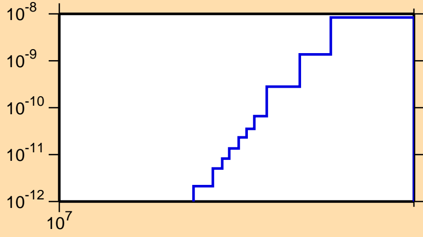
\sigma vs. E for ^{145}\text{Dy}(\text{mt117})
