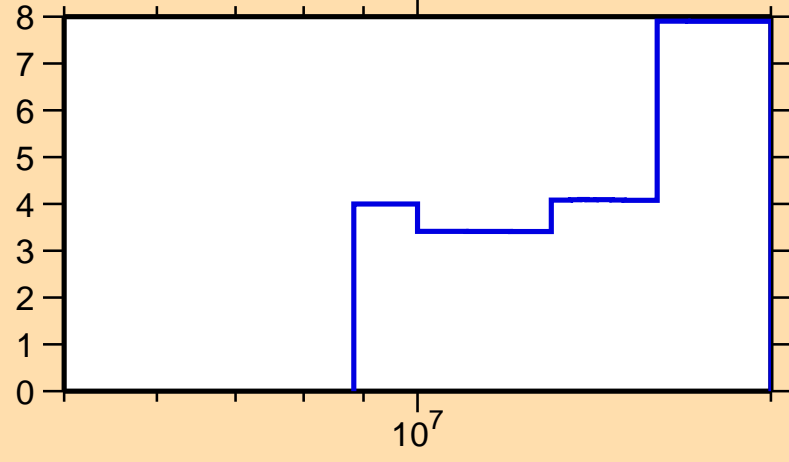
\Delta\sigma/\sigma vs. E for ^{145}\text{Dy}(n,\text{tot.})
